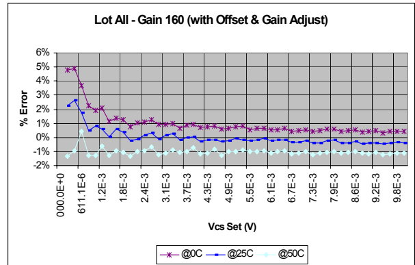
FIGURE 21. AVERAGE INPUT TO OUTPUT ERROR WITH CORRECTION FOR OFFSET AND GAIN FOR EACH INPUT VOLTAGE AT 0°C, 25°C AND 50°C
