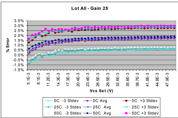
FIGURE 10. INPUT TO OUTPUT % ERROR (EXPANDED - STARTS AT 5mV INPUT). THIS IS THE RAW ERROR WITH NO CORRECTION FOR OFFSET OR GAIN. IT INCLUDES ERROR AT EACH TEMPERATURE WITH THREE STANDARD DEVIATIONS
