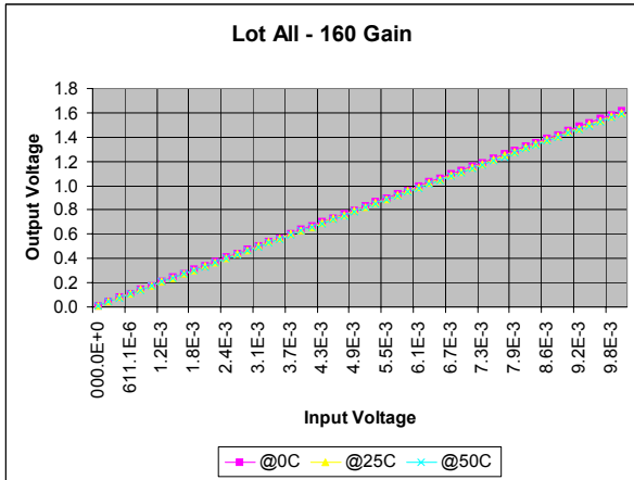
FIGURE 18. INPUT TO OUTPUT VOLTAGE
