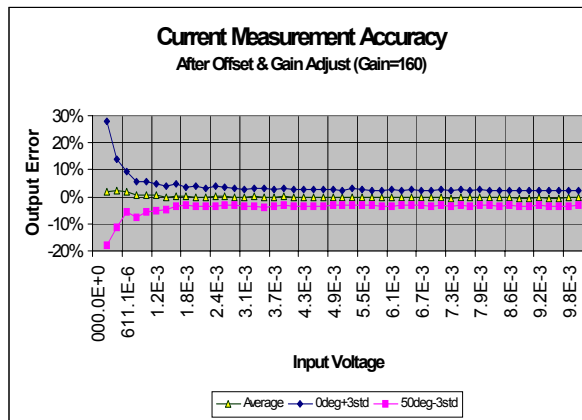
FIGURE 22. WORST CASE INPUT TO OUTPUT ERROR WITH CORRECTION FOR OFFSET AND GAIN. THE TERM +3 STDEV IS WORST CASE VALUE FOR 0°C. THE TERM -3 STDEV IS THE WORST CASE VALUE FOR 50°C
