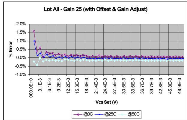
FIGURE 11. AVERAGE INPUT TO OUTPUT ERROR WITH CORRECTION FOR OFFSET AND GAIN FOR EACH INPUT VOLTAGE AT 0°C, 25°C AND 50°C
