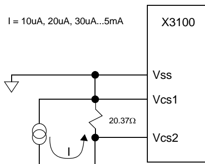
FIGURE 1. CURRENT SENSE MEASUREMENT
