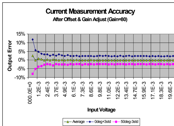
FIGURE 17. WORST CASE INPUT TO OUTPUT ERROR WITH CORRECTION FOR OFFSET AND GAIN. THE TERM +3 STDEV IS WORST CASE VALUE FOR 0°C. THE TERM -3 STDEV IS THE WORST CASE VALUE FOR 50°C
