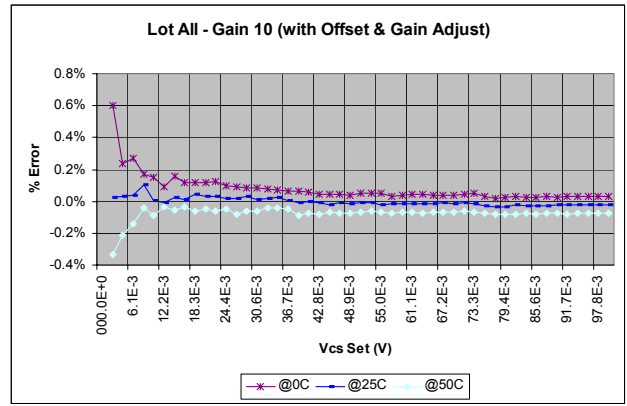
FIGURE 6. AVERAGE INPUT TO OUTPUT ERROR WITH CORRECTION FOR OFFSET AND GAIN FOR EACH INPUT VOLTAGE AT 0°C, 25°C AND 50°C
