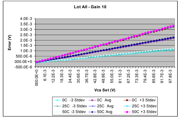
FIGURE 4. INPUT TO OUTPUT ERROR. THIS IS THE RAW ERROR WITH NO CORRECTION FOR OFFSET OR GAIN. IT INCLUDES ERROR AT EACH TEMPERATURE WITH THREE STANDARD DEVIATIONS
