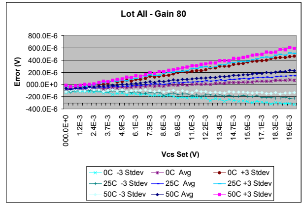
FIGURE 14. INPUT TO OUTPUT ERROR. THIS IS THE RAW ERROR WITH NO CORRECTION FOR OFFSET OR GAIN. IT INCLUDES ERROR AT EACH TEMPERATURE WITH THREE STANDARD DEVIATIONS
