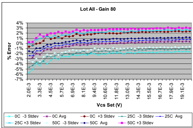
FIGURE 15. INPUT TO OUTPUT % ERROR (EXPANDED - STARTS AT 2mV INPUT). THIS IS THE RAW ERROR WITH NO CORRECTION FOR OFFSET OR GAIN. IT INCLUDES ERROR AT EACH TEMPERATURE WITH THREE STANDARD DEVIATIONS
