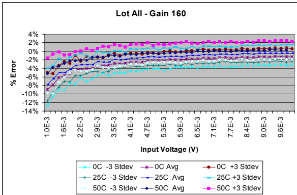
FIGURE 20. INPUT TO OUTPUT % ERROR (EXPANDED - STARTS AT 1mV INPUT). THIS IS THE RAW ERROR WITH NO CORRECTION FOR OFFSET OR GAIN. IT INCLUDES ERROR AT EACH TEMPERATURE WITH THREE STANDARD DEVIATIONS
