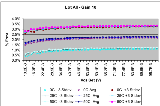
FIGURE 5. INPUT TO OUTPUT % ERROR (EXPANDED - STARTS AT 10mV INPUT). THIS IS THE RAW ERROR WITH NO CORRECTION FOR OFFSET OR GAIN. IT INCLUDES ERROR AT EACH TEMPERATURE WITH THREE STANDARD DEVIATIONS
