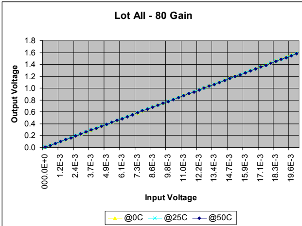
FIGURE 13. INPUT TO OUTPUT VOLTAGE
