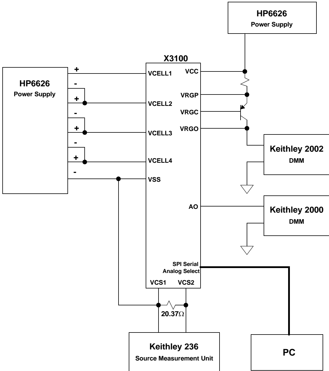
FIGURE 2. CHARACTERIZATION TEST SETUP
