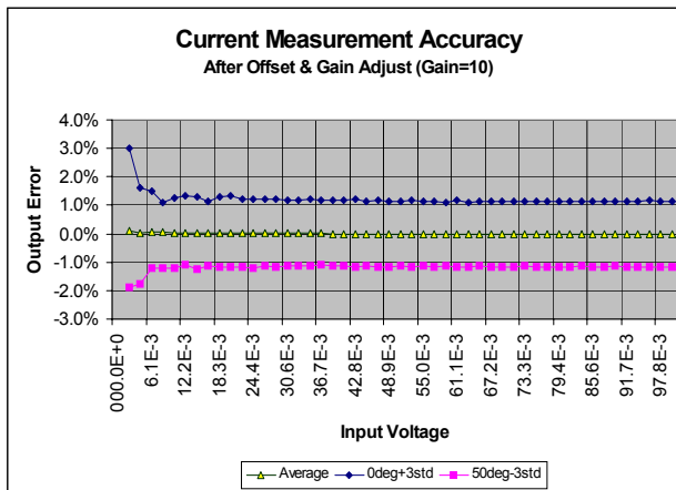
FIGURE 7. WORST CASE INPUT TO OUTPUT ERROR WITH CORRECTION FOR OFFSET AND GAIN. THE TERM +3 STDEV IS THE WORST CASE VALUE FOR 0°C. THE TERM -3 STDEV IS THE WORST CASE VALUE FOR 50°C
