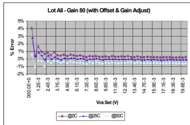
FIGURE 16. AVERAGE INPUT TO OUTPUT ERROR WITH CORRECTION FOR OFFSET AND GAIN FOR EACH INPUT VOLTAGE AT 0°C, 25°C AND 50°C
