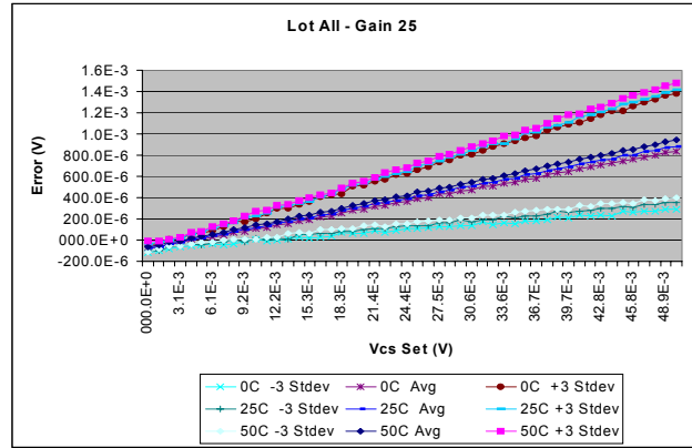
FIGURE 9. INPUT TO OUTPUT ERROR. THIS IS THE RAW ERROR WITH NO CORRECTION FOR OFFSET OR GAIN. IT INCLUDES ERROR AT EACH TEMPERATURE WITH THREE STANDARD DEVIATIONS
