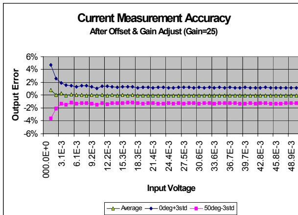
FIGURE 12. WORST CASE INPUT TO OUTPUT ERROR WITH CORRECTION FOR OFFSET AND GAIN. THE TERM +3 STDEV IS WORST CASE VALUE FOR 0°C. THE TERM -3 STDEV IS THE WORST CASE VALUE FOR 50°C
