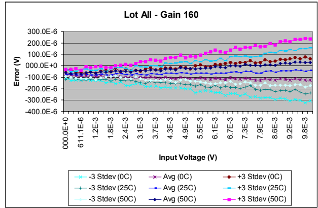
FIGURE 19. INPUT TO OUTPUT ERROR. THIS IS THE RAW ERROR WITH NO CORRECTION FOR OFFSET OR GAIN. IT INCLUDES ERROR AT EACH TEMPERATURE WITH THREE STANDARD DEVIATIONS
