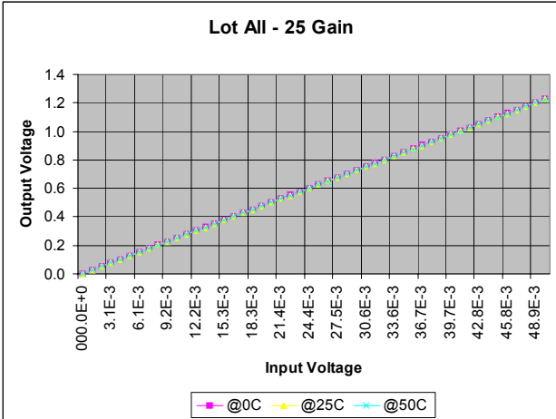
FIGURE 8. INPUT TO OUTPUT VOLTAGE
