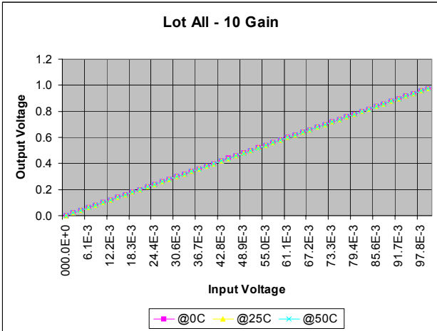
FIGURE 3. INPUT TO OUTPUT VOLTAGE
